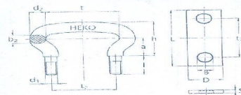
Figure 21: HEKO chain shackle type S
